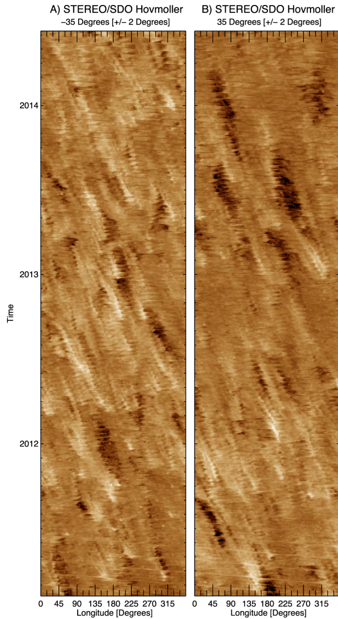
Figure 2. from The Longitudinal Evolution of Equatorial Coronal Holes null 2018 AJ 155 153 doi:10.3847/1538-3881/aaaebf https://dx.doi.org/10.3847/1538-3881/aaaebf © 2018. The American Astronomical Society. All rights reserved.
