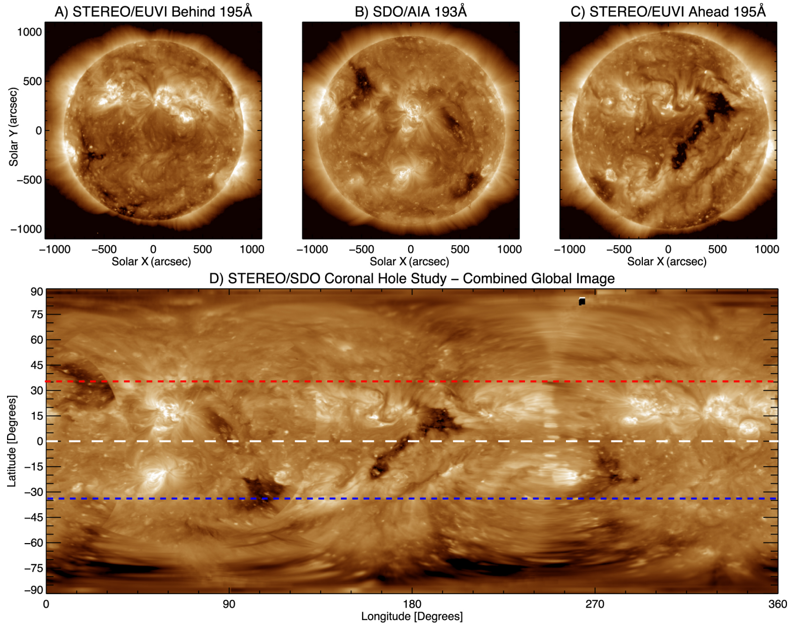
Figure 1. from The Longitudinal Evolution of Equatorial Coronal Holes null 2018 AJ 155 153 doi:10.3847/1538-3881/aaaebf https://dx.doi.org/10.3847/1538-3881/aaaebf © 2018. The American Astronomical Society. All rights reserved.
