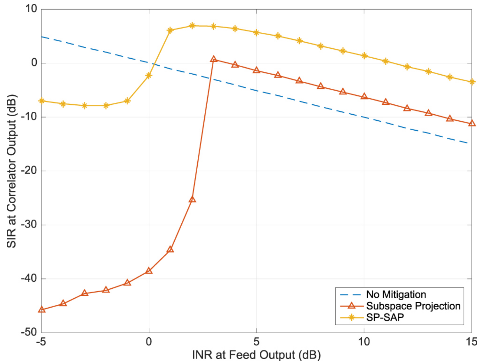
Figure 6. from Subarray Processing for Projection-based RFI Mitigation in Radio Astronomical Interferometers null 2018 AJ 155 146 doi:10.3847/1538-3881/aaae6f https://dx.doi.org/10.3847/1538-3881/aaae6f © 2018. The American Astronomical Society. All rights reserved.
