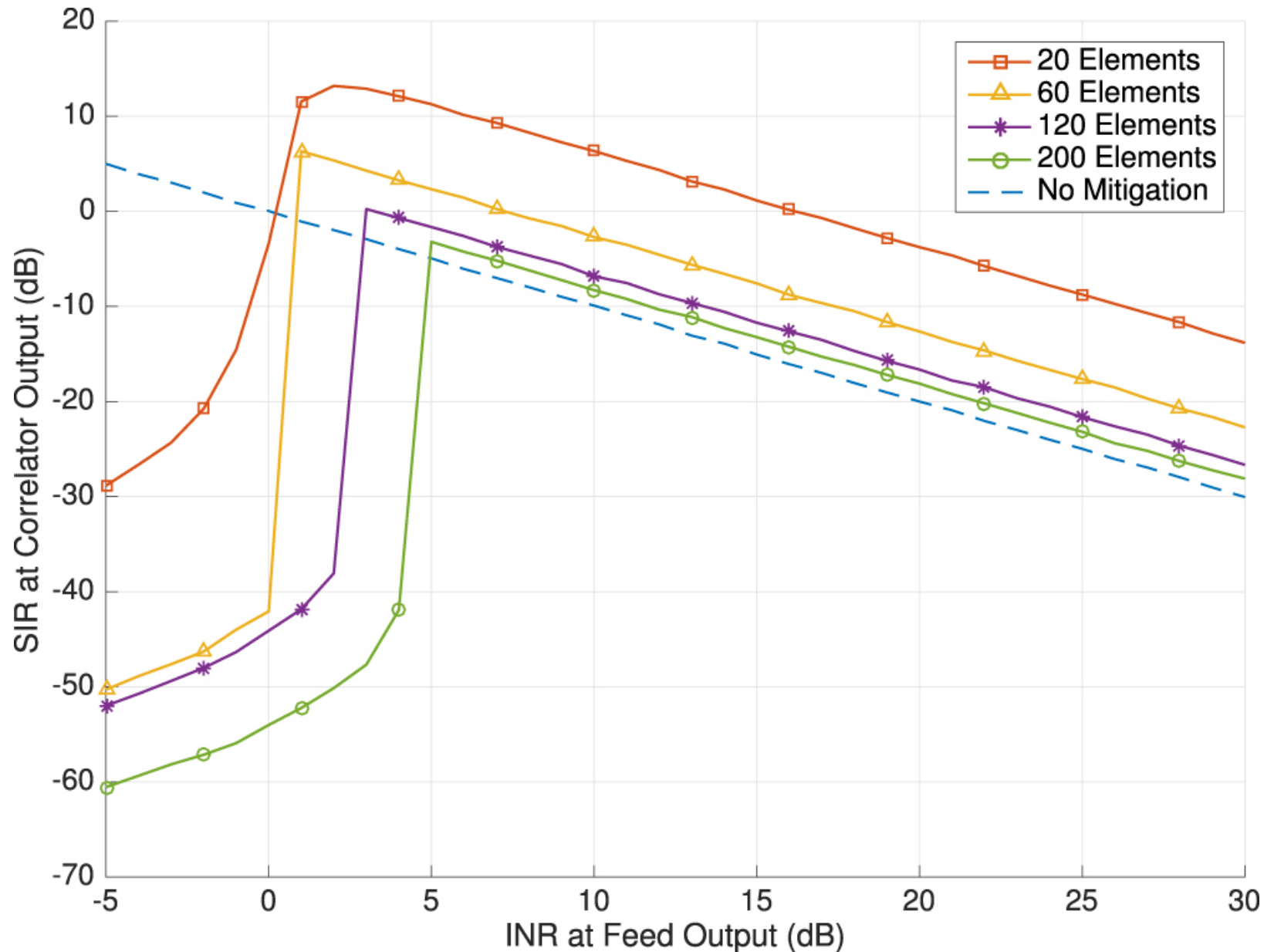
Figure 4. from Subarray Processing for Projection-based RFI Mitigation in Radio Astronomical Interferometers null 2018 AJ 155 146 doi:10.3847/1538-3881/aaae6f https://dx.doi.org/10.3847/1538-3881/aaae6f © 2018. The American Astronomical Society. All rights reserved.
