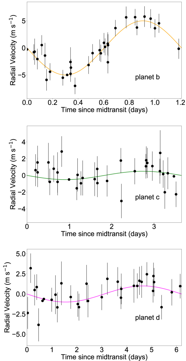
Figure 9. from Magellan/PFS Radial Velocities of GJ 9827, a Late K dwarf at 30 pc with Three Transiting Super-Earths null 2018 AJ 155 148 doi:10.3847/1538-3881/aaab56 https://dx.doi.org/10.3847/1538-3881/aaab56 © 2018. The American Astronomical Society. All rights reserved.
