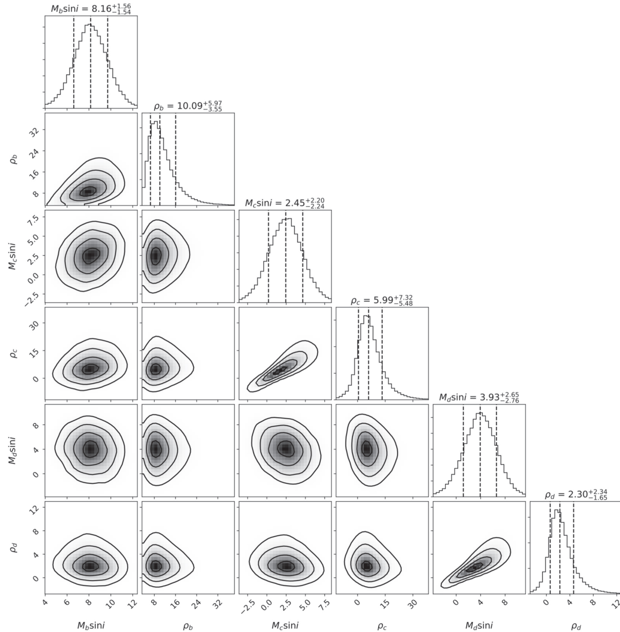
Figure 7. from Magellan/PFS Radial Velocities of GJ 9827, a Late K dwarf at 30 pc with Three Transiting Super-Earths null 2018 AJ 155 148 doi:10.3847/1538-3881/aaab56 https://dx.doi.org/10.3847/1538-3881/aaab56 © 2018. The American Astronomical Society. All rights reserved.
