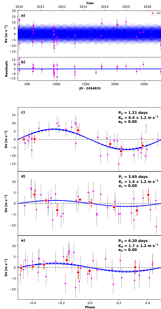
Figure 5. from Magellan/PFS Radial Velocities of GJ 9827, a Late K dwarf at 30 pc with Three Transiting Super-Earths null 2018 AJ 155 148 doi:10.3847/1538-3881/aaab56 https://dx.doi.org/10.3847/1538-3881/aaab56 © 2018. The American Astronomical Society. All rights reserved.
