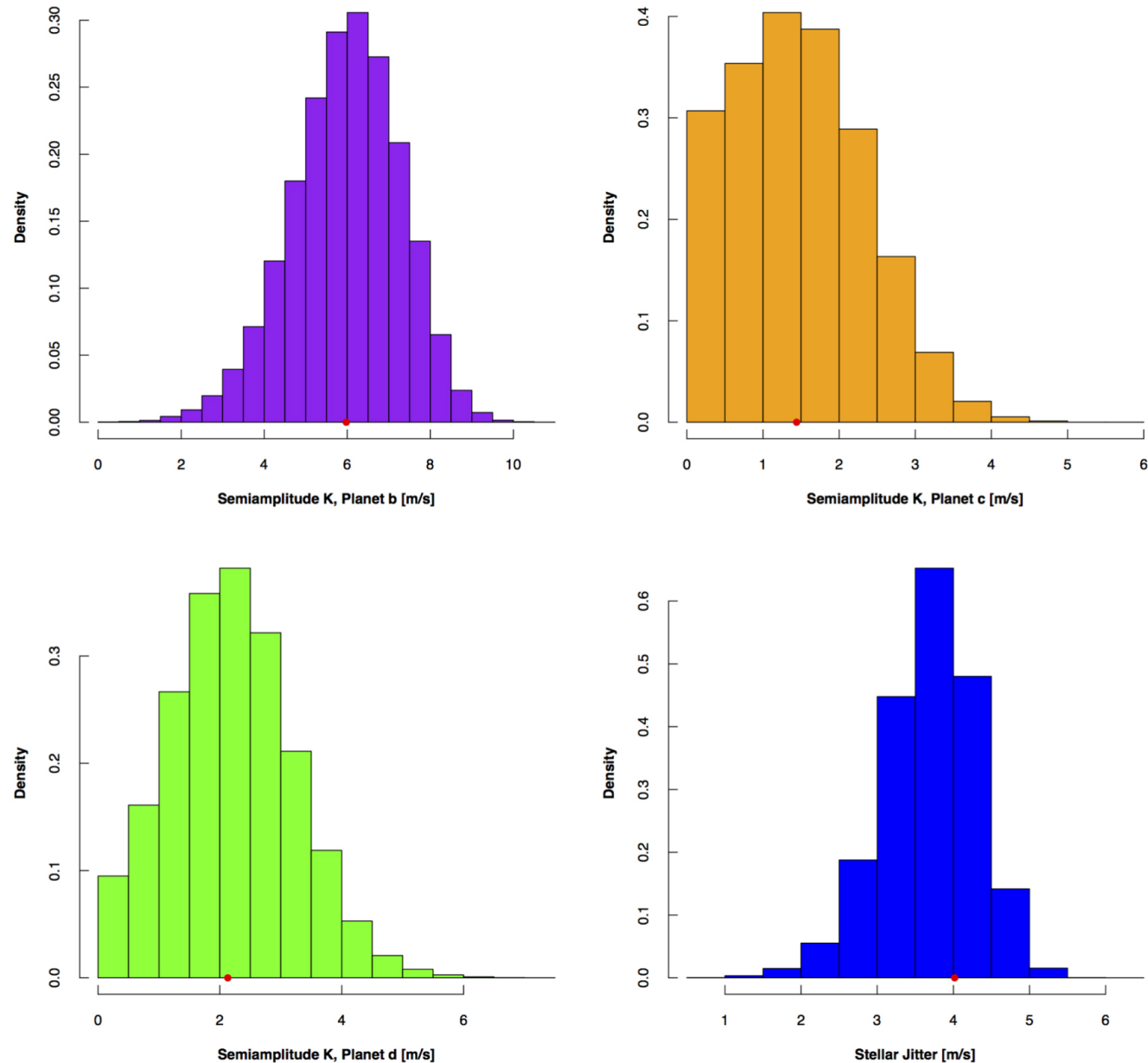
Figure 4. from Magellan/PFS Radial Velocities of GJ 9827, a Late K dwarf at 30 pc with Three Transiting Super-Earths null 2018 AJ 155 148 doi:10.3847/1538-3881/aaab56 https://dx.doi.org/10.3847/1538-3881/aaab56
