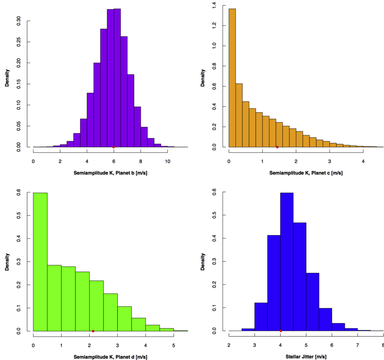
Figure 3. from Magellan/PFS Radial Velocities of GJ 9827, a Late K dwarf at 30 pc with Three Transiting Super-Earths null 2018 AJ 155 148 doi:10.3847/1538-3881/aaab56 https://dx.doi.org/10.3847/1538-3881/aaab56 © 2018. The American Astronomical Society. All rights reserved.
