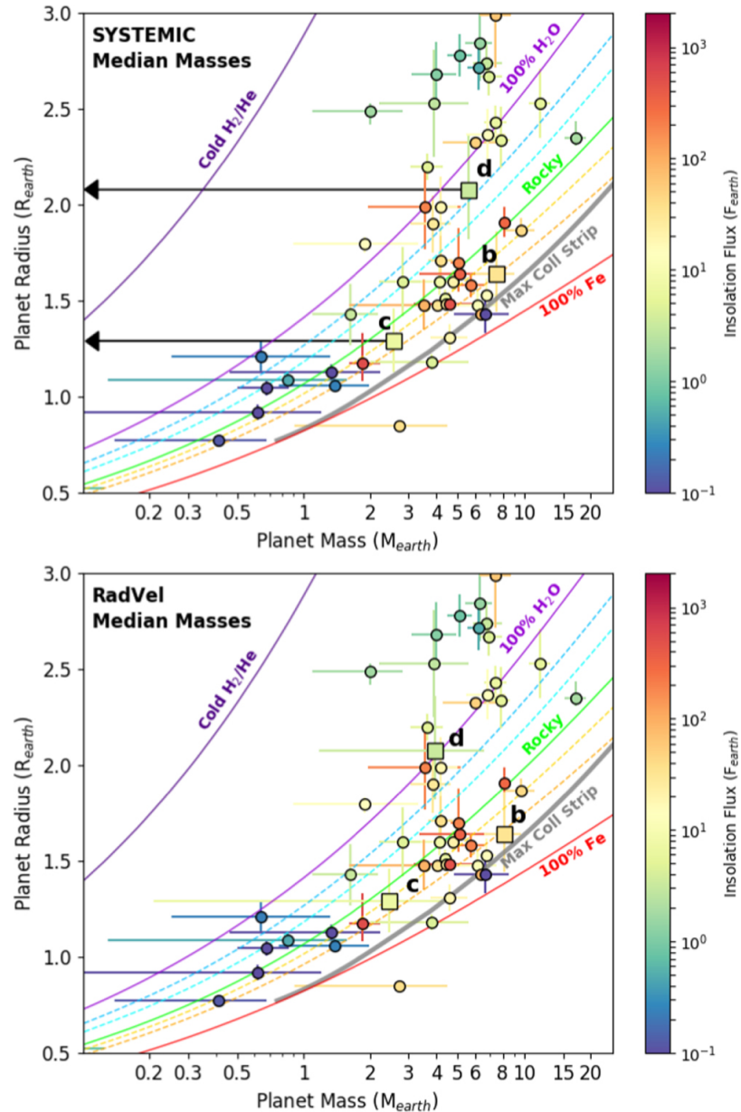
Figure 10. from Magellan/PFS Radial Velocities of GJ 9827, a Late K dwarf at 30 pc with Three Transiting Super-Earths null 2018 AJ 155 148 doi:10.3847/1538-3881/aaab56 https://dx.doi.org/10.3847/1538-3881/aaab56
