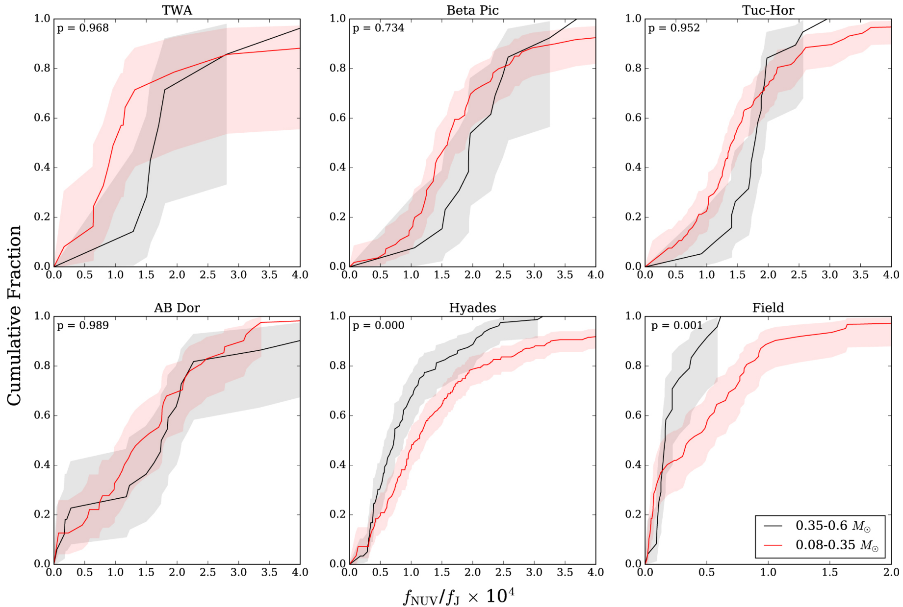
Figure 7. from HAZMAT. III. The UV Evolution of Mid- to Late-M Stars with GALEX null 2018 AJ 155 122 doi:10.3847/1538-3881/aaaa24 https://dx.doi.org/10.3847/1538-3881/aaaa24 © 2018. The American Astronomical Society. All rights reserved.
