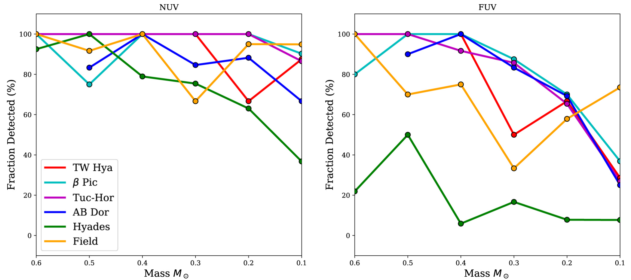
Figure 2. from HAZMAT. III. The UV Evolution of Mid- to Late-M Stars with GALEX null 2018 AJ 155 122 doi:10.3847/1538-3881/aaaa24 https://dx.doi.org/10.3847/1538-3881/aaaa24 © 2018. The American Astronomical Society. All rights reserved.
