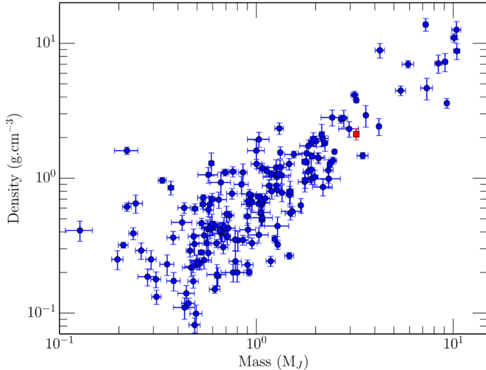
Figure 9. from HATS-36b and 24 Other Transiting/Eclipsing Systems from the HATSouth-K2 Campaign 7 Program null 2018 AJ 155 119 doi:10.3847/1538-3881/aaa8e6 https://dx.doi.org/10.3847/1538-3881/aaa8e6 © 2018. The American Astronomical Society. All rights reserved.
