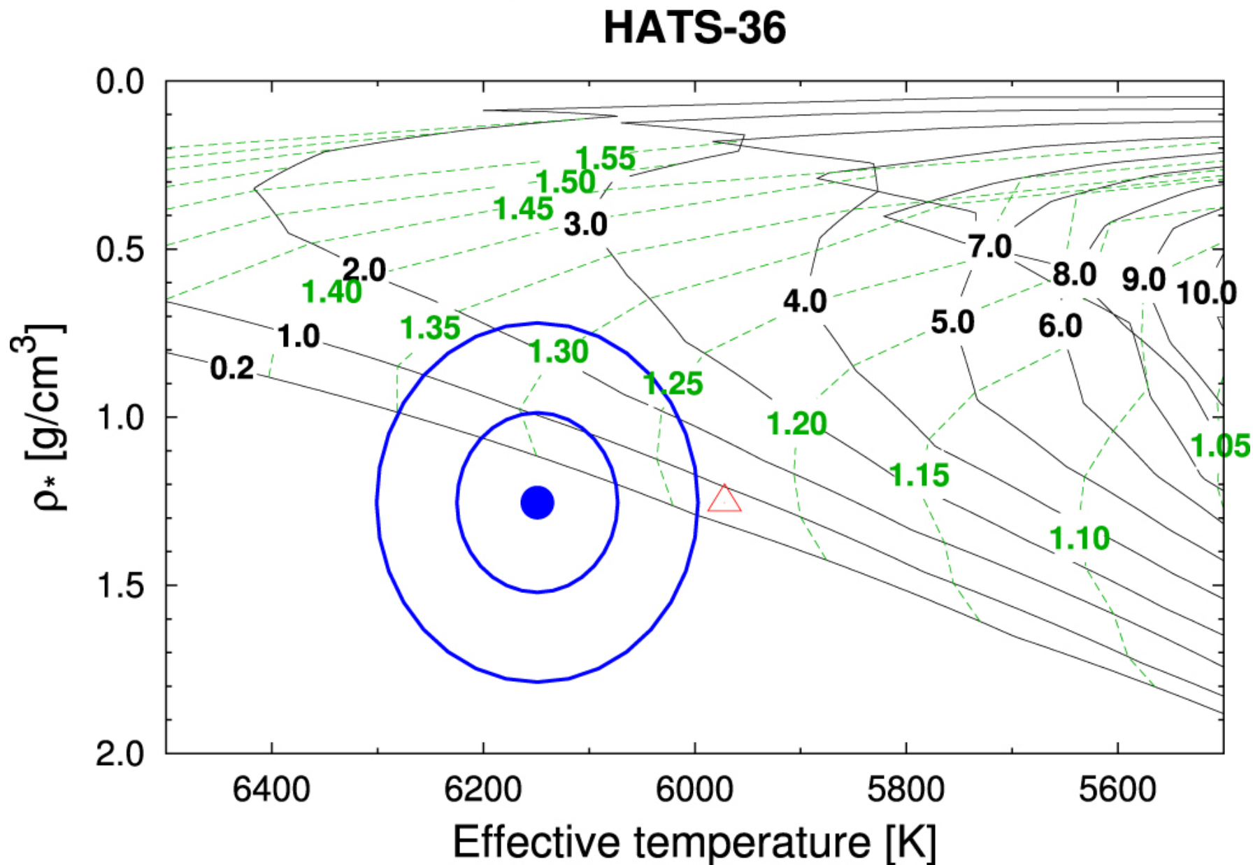
Figure 7. from HATS-36b and 24 Other Transiting/Eclipsing Systems from the HATSouth-K2 Campaign 7 Program null 2018 AJ 155 119 doi:10.3847/1538-3881/aaa8e6 https://dx.doi.org/10.3847/1538-3881/aaa8e6 © 2018. The American Astronomical Society. All rights reserved.
