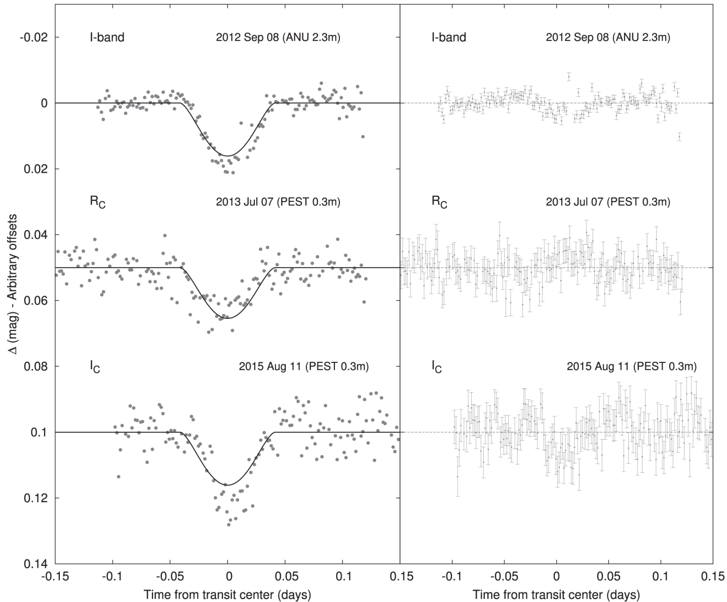
Figure 3. from HATS-36b and 24 Other Transiting/Eclipsing Systems from the HATSouth-K2 Campaign 7 Program null 2018 AJ 155 119 doi:10.3847/1538-3881/aaa8e6 https://dx.doi.org/10.3847/1538-3881/aaa8e6 © 2018. The American Astronomical Society. All rights reserved.
