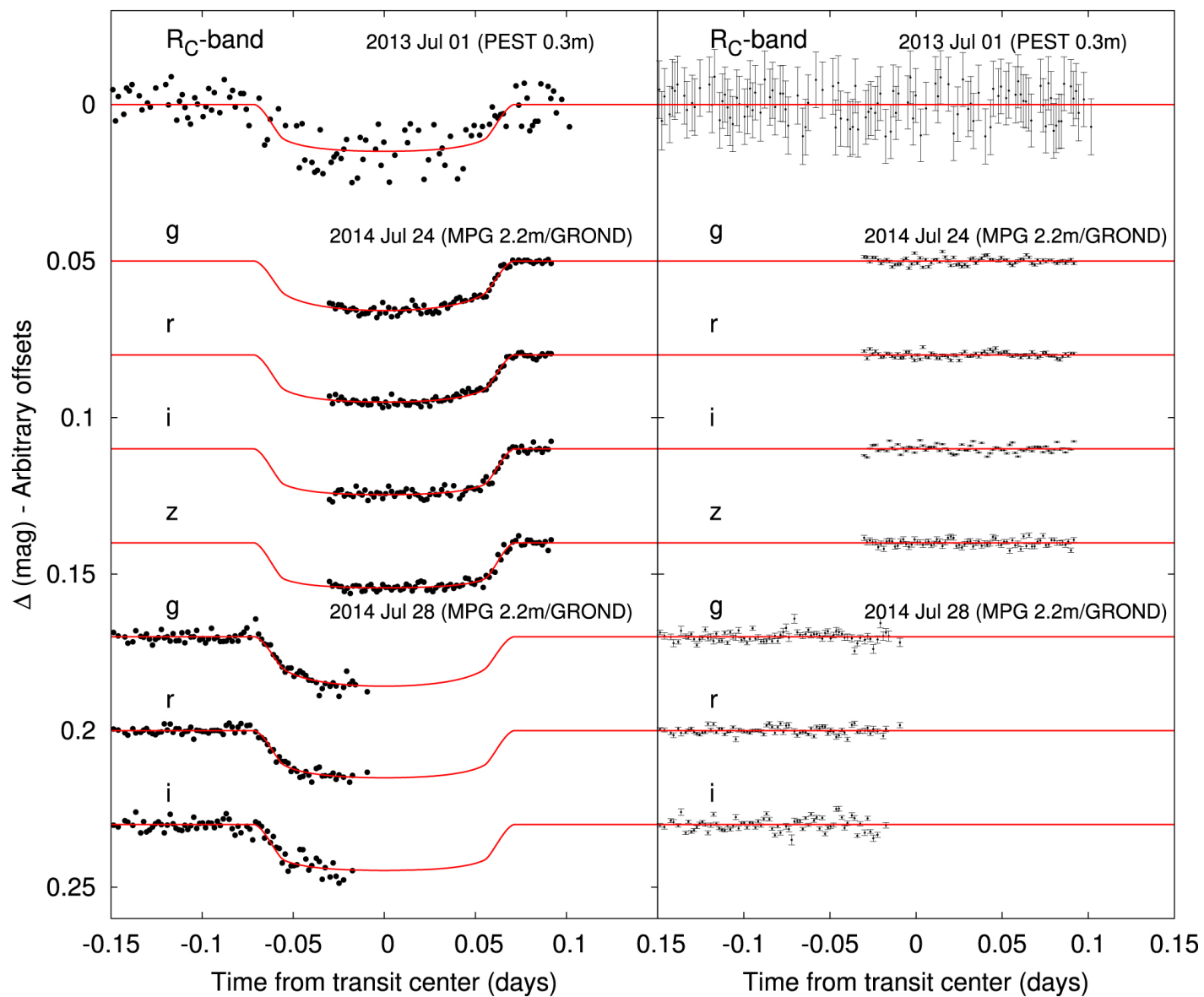
Figure 2. from HATS-36b and 24 Other Transiting/Eclipsing Systems from the HATSouth-K2 Campaign 7 Program null 2018 AJ 155 119 doi:10.3847/1538-3881/aaa8e6 https://dx.doi.org/10.3847/1538-3881/aaa8e6 © 2018. The American Astronomical Society. All rights reserved.
