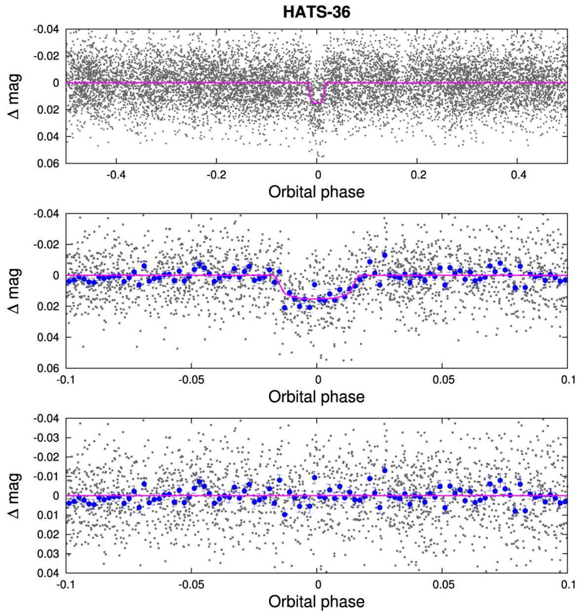
Figure 1. from HATS-36b and 24 Other Transiting/Eclipsing Systems from the HATSouth-K2 Campaign 7 Program null 2018 AJ 155 119 doi:10.3847/1538-3881/aaa8e6 https://dx.doi.org/10.3847/1538-3881/aaa8e6 © 2018. The American Astronomical Society. All rights reserved.
