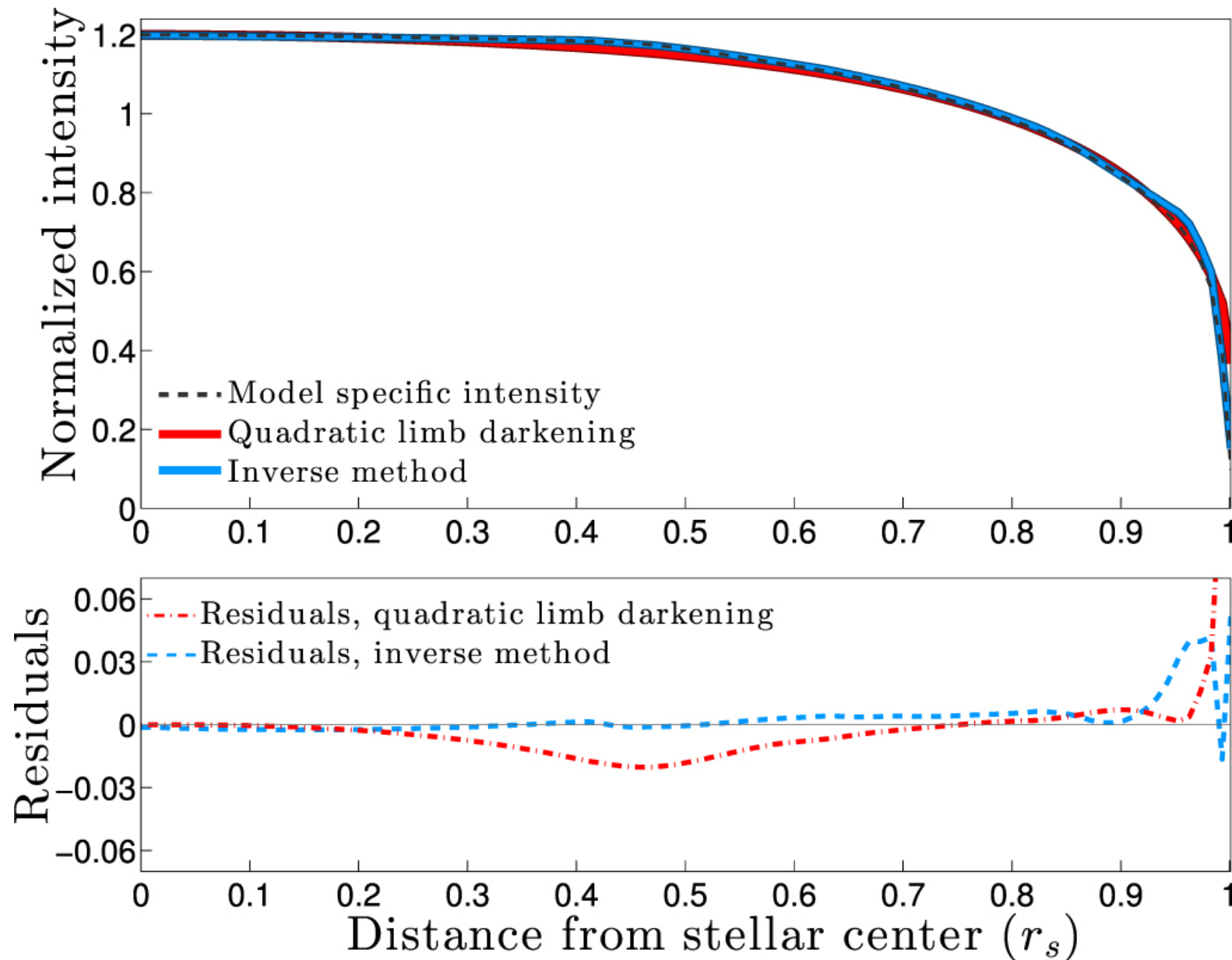
Figure 8. from Model-independent Exoplanet Transit Spectroscopy null 2018 AJ 155 208 doi:10.3847/1538-3881/aaa3fe https://dx.doi.org/10.3847/1538-3881/aaa3fe © 2018. The American Astronomical Society. All rights reserved.
