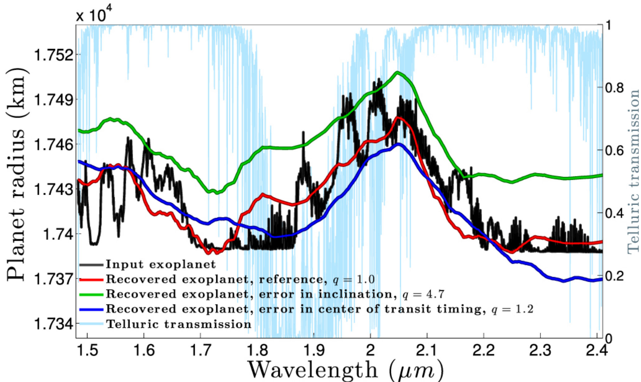
Figure 6. from Model-independent Exoplanet Transit Spectroscopy null 2018 AJ 155 208 doi:10.3847/1538-3881/aaa3fe https://dx.doi.org/10.3847/1538-3881/aaa3fe © 2018. The American Astronomical Society. All rights reserved.
