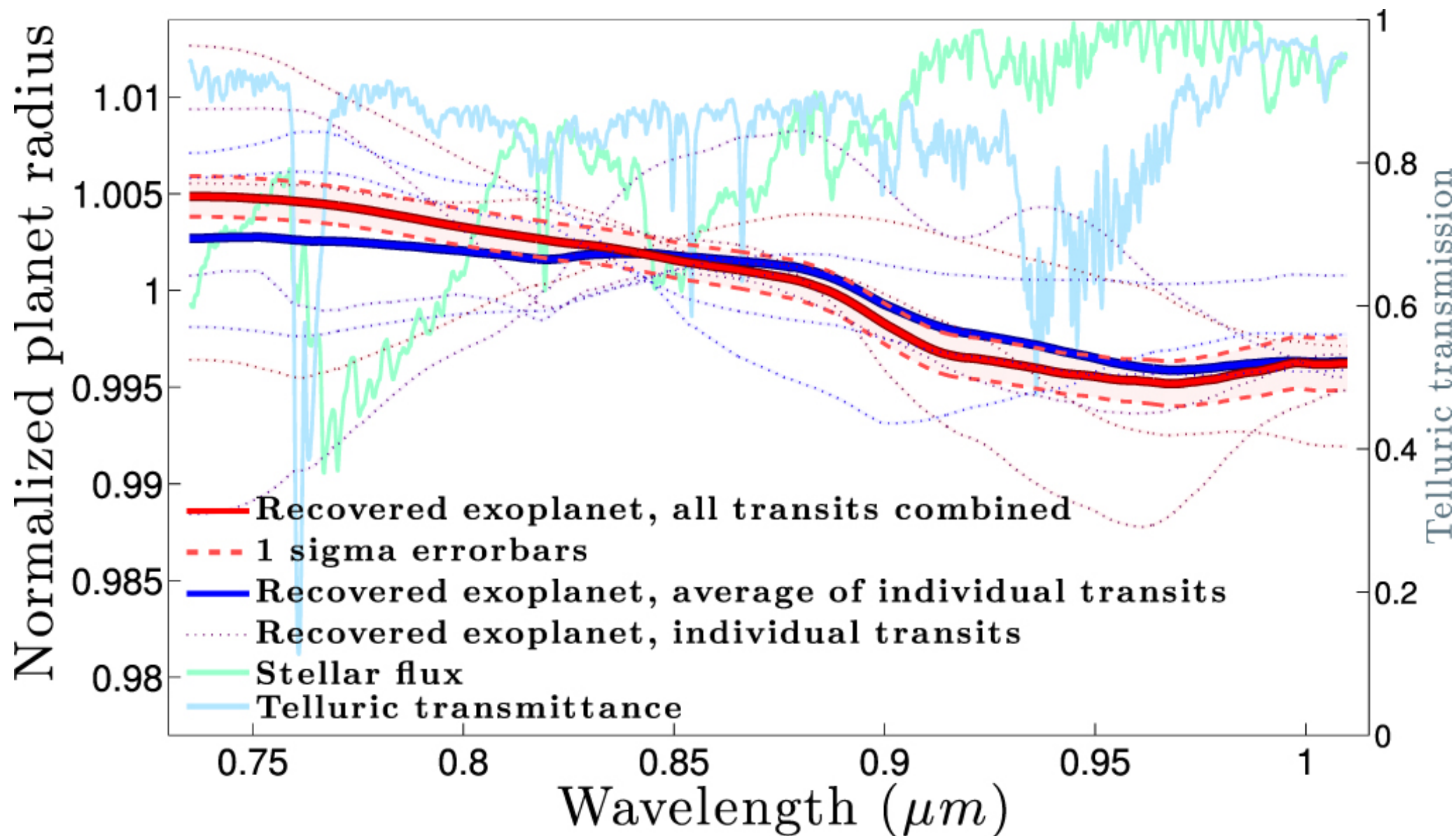
Figure 14. from Model-independent Exoplanet Transit Spectroscopy null 2018 AJ 155 208 doi:10.3847/1538-3881/aaa3fe https://dx.doi.org/10.3847/1538-3881/aaa3fe © 2018. The American Astronomical Society. All rights reserved.
