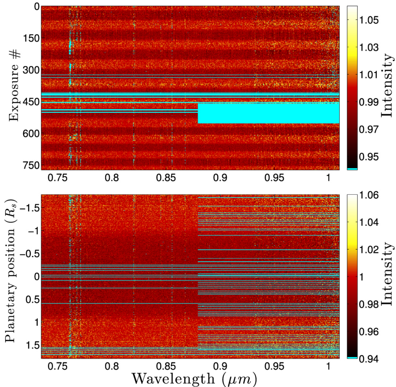
Figure 13. from Model-independent Exoplanet Transit Spectroscopy null 2018 AJ 155 208 doi:10.3847/1538-3881/aaa3fe https://dx.doi.org/10.3847/1538-3881/aaa3fe © 2018. The American Astronomical Society. All rights reserved.
