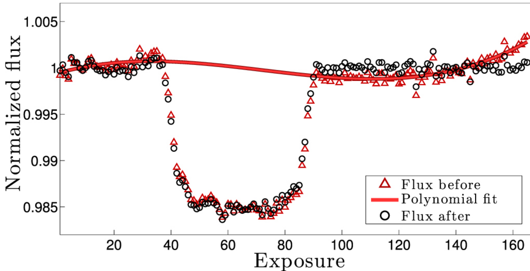
Figure 12. from Model-independent Exoplanet Transit Spectroscopy null 2018 AJ 155 208 doi:10.3847/1538-3881/aaa3fe https://dx.doi.org/10.3847/1538-3881/aaa3fe © 2018. The American Astronomical Society. All rights reserved.
