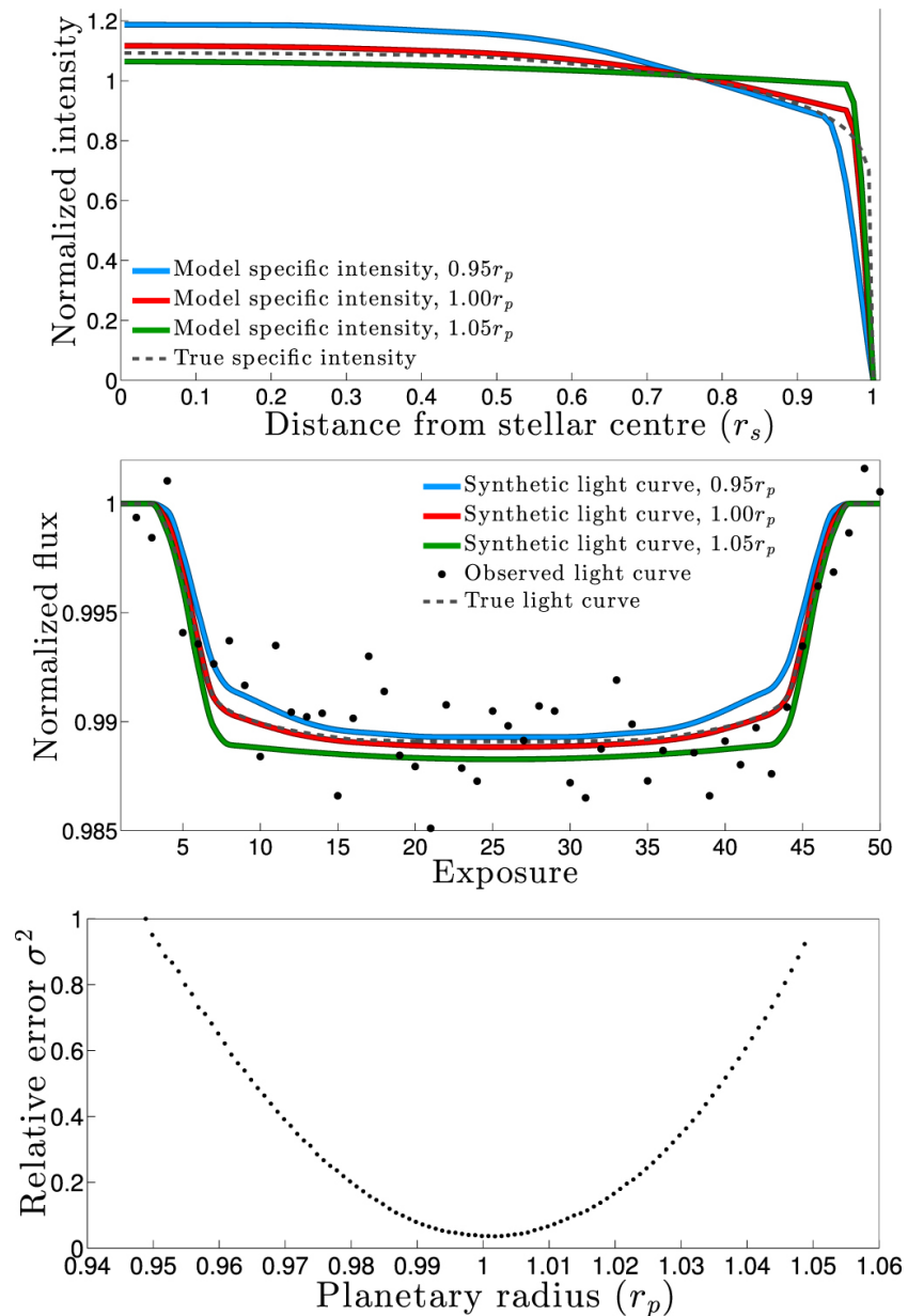
Figure 1. from Model-independent Exoplanet Transit Spectroscopy null 2018 AJ 155 208 doi:10.3847/1538-3881/aaa3fe https://dx.doi.org/10.3847/1538-3881/aaa3fe © 2018. The American Astronomical Society. All rights reserved.
