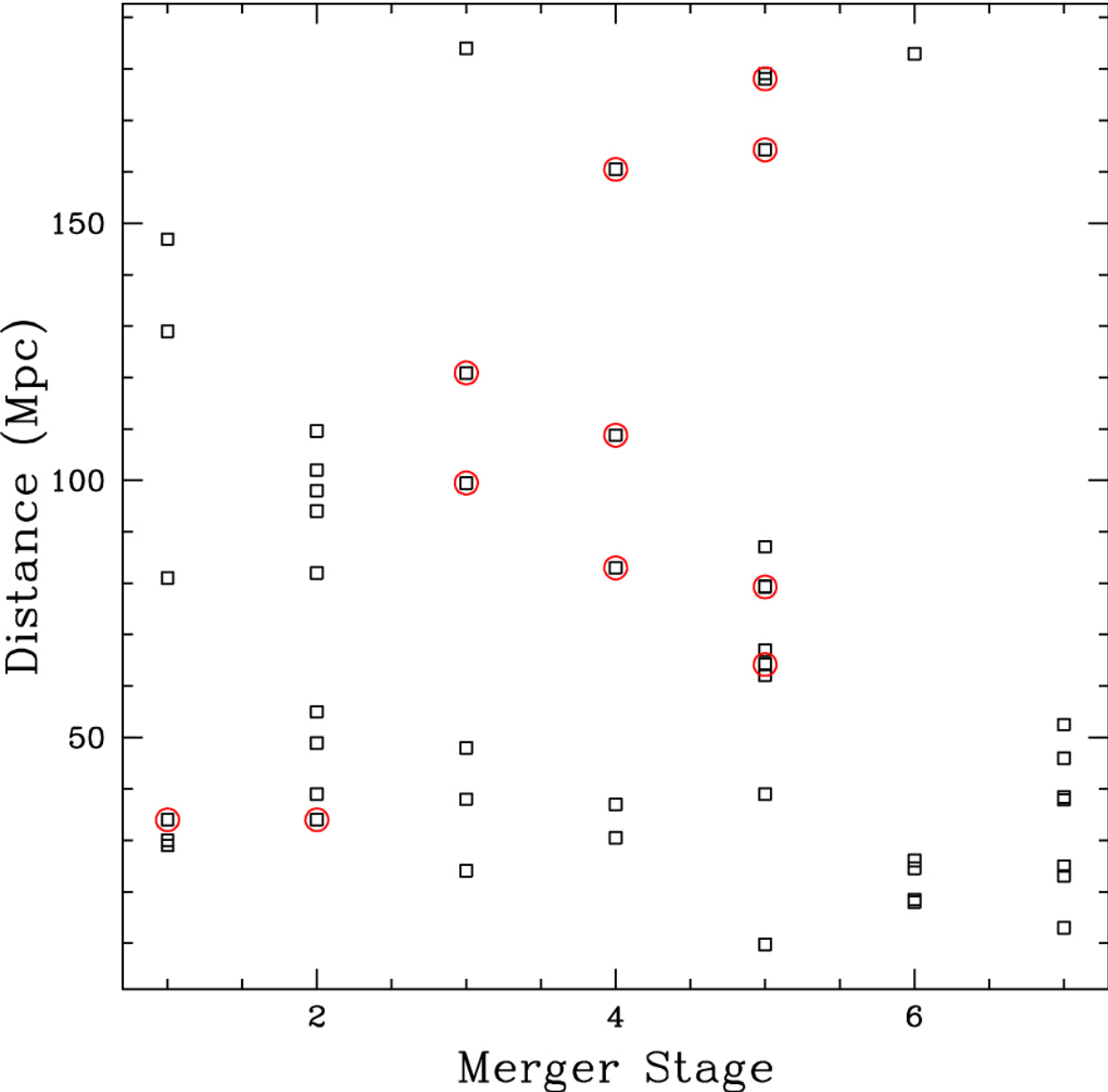
Figure 2. from Diffuse X-Ray-emitting Gas in Major Mergers null 2018 AJ 155 81 doi:10.3847/1538-3881/aaa1a6 https://dx.doi.org/10.3847/1538-3881/aaa1a6 © 2018. The American Astronomical Society. All rights reserved.
