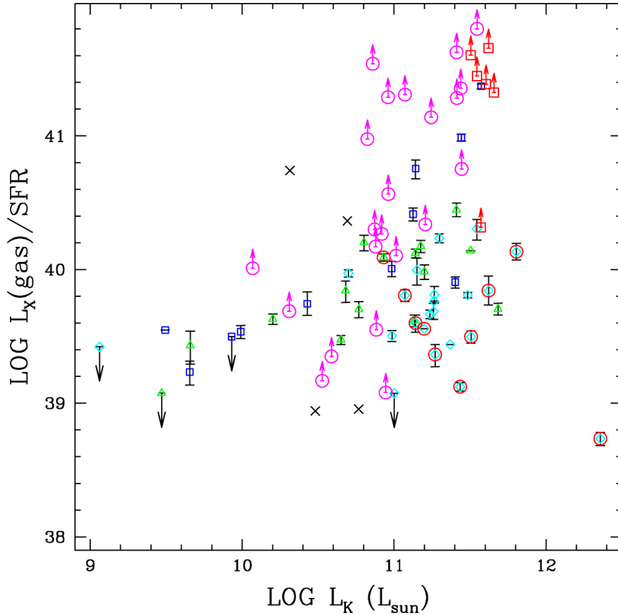
Figure 13. from Diffuse X-Ray-emitting Gas in Major Mergers null 2018 AJ 155 81 doi:10.3847/1538-3881/aaa1a6 https://dx.doi.org/10.3847/1538-3881/aaa1a6 © 2018. The American Astronomical Society. All rights reserved.
