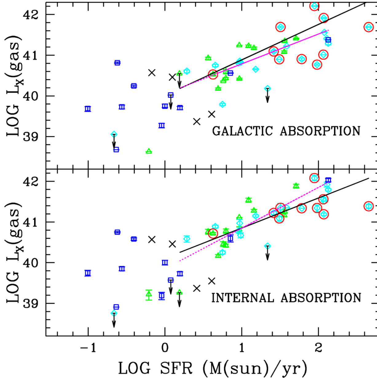
Figure 12. from Diffuse X-Ray-emitting Gas in Major Mergers null 2018 AJ 155 81 doi:10.3847/1538-3881/aaa1a6 https://dx.doi.org/10.3847/1538-3881/aaa1a6 © 2018. The American Astronomical Society. All rights reserved.
