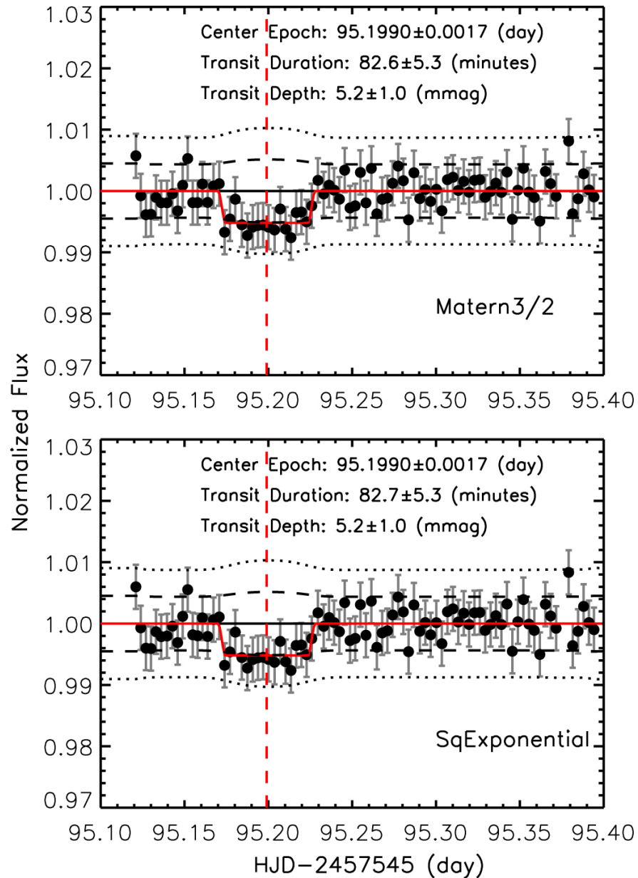
Figure 6. from Searching for the Transit of the Earth-mass Exoplanet Proxima Centauri b in Antarctica: Preliminary Result null 2018 AJ 155 12 doi:10.3847/1538-3881/aa9b86 https://dx.doi.org/10.3847/1538-3881/aa9b86
