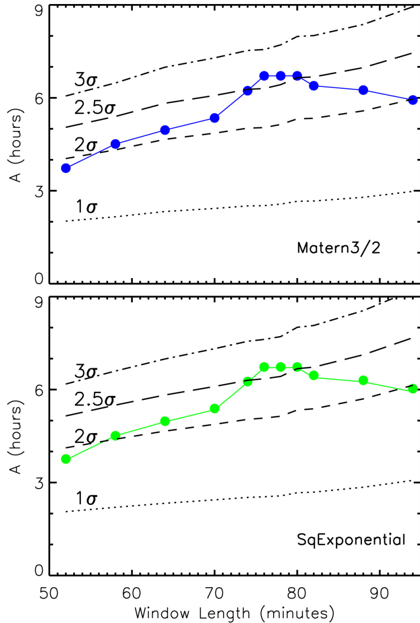
Figure 5. from Searching for the Transit of the Earth-mass Exoplanet Proxima Centauri b in Antarctica: Preliminary Result null 2018 AJ 155 12 doi:10.3847/1538-3881/aa9b86 https://dx.doi.org/10.3847/1538-3881/aa9b86 © 2017. The American Astronomical Society. All rights reserved.
