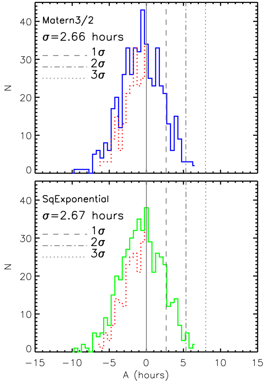
Figure 4. from Searching for the Transit of the Earth-mass Exoplanet Proxima Centauri b in Antarctica: Preliminary Result null 2018 AJ 155 12 doi:10.3847/1538-3881/aa9b86 https://dx.doi.org/10.3847/1538-3881/aa9b86 © 2017. The American Astronomical Society. All rights reserved.
