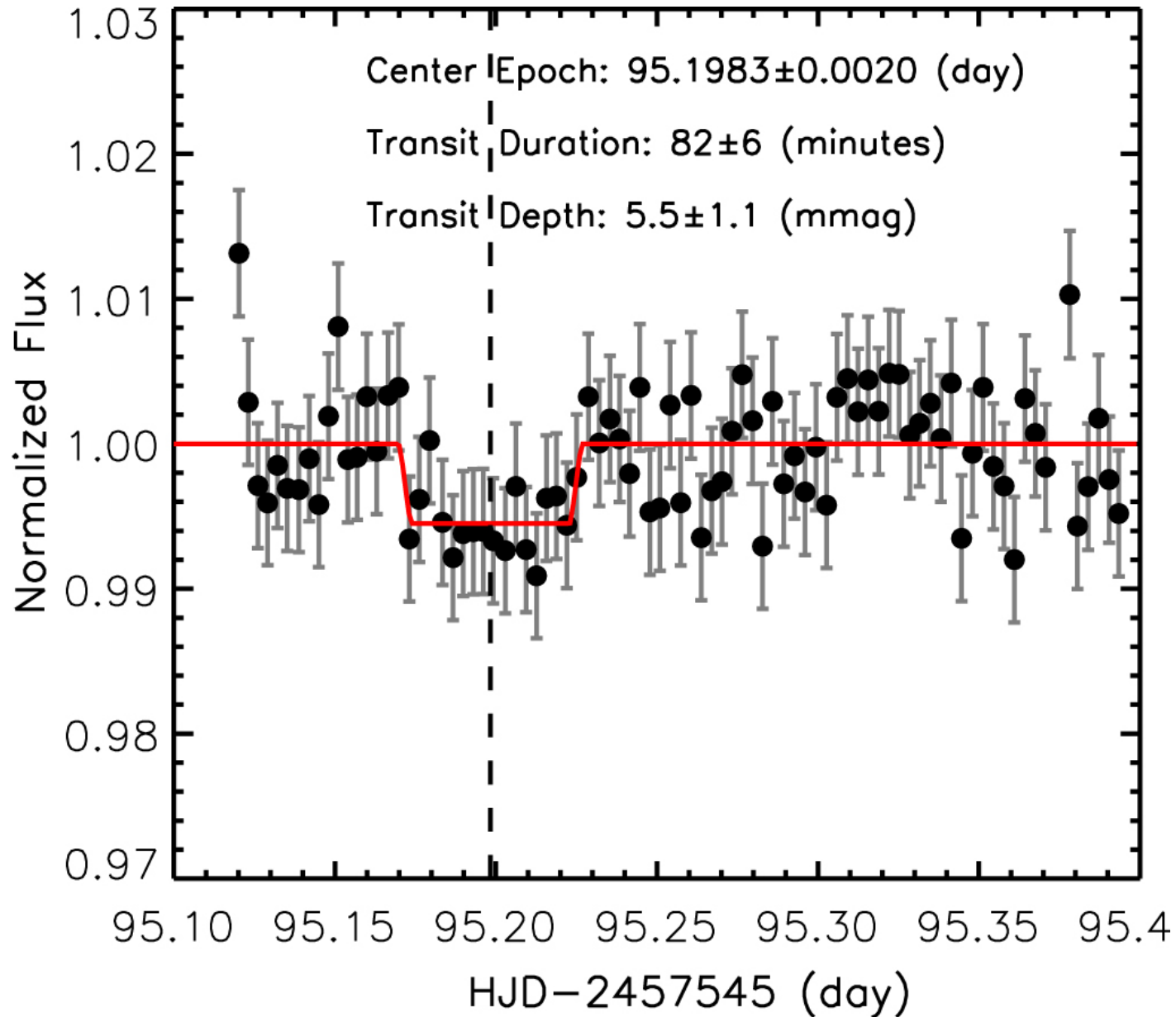
Figure 2. from Searching for the Transit of the Earth-mass Exoplanet Proxima Centauri b in Antarctica: Preliminary Result null 2018 AJ 155 12 doi:10.3847/1538-3881/aa9b86 https://dx.doi.org/10.3847/1538-3881/aa9b86 © 2017. The American Astronomical Society. All rights reserved.
