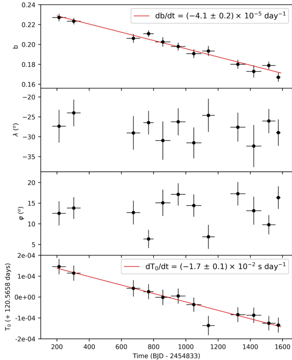
Figure 5. from Spin–Orbit Misalignment and Precession in the Kepler-13Ab Planetary System null 2018 AJ 155 13 doi:10.3847/1538-3881/aa991f https://dx.doi.org/10.3847/1538-3881/aa991f © 2017. The American Astronomical Society. All rights reserved.
