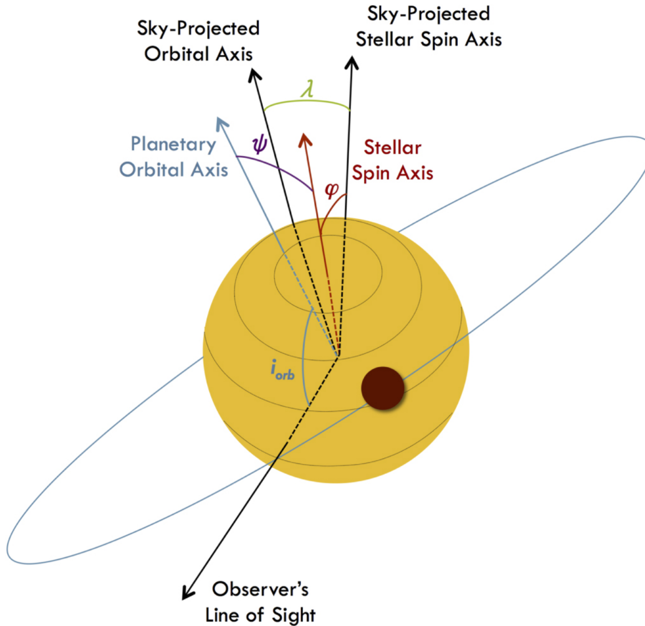
Figure 3. from Spin–Orbit Misalignment and Precession in the Kepler-13Ab Planetary System null 2018 AJ 155 13 doi:10.3847/1538-3881/aa991f https://dx.doi.org/10.3847/1538-3881/aa991f © 2017. The American Astronomical Society. All rights reserved.
