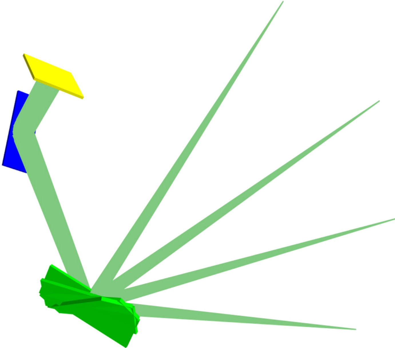
Figure 3. from MARXS: A Modular Software to Ray-trace X-Ray Instrumentation null 2017 AJ 154 243 doi:10.3847/1538-3881/aa943b https://dx.doi.org/10.3847/1538-3881/aa943b © 2017. The American Astronomical Society. All rights reserved.
