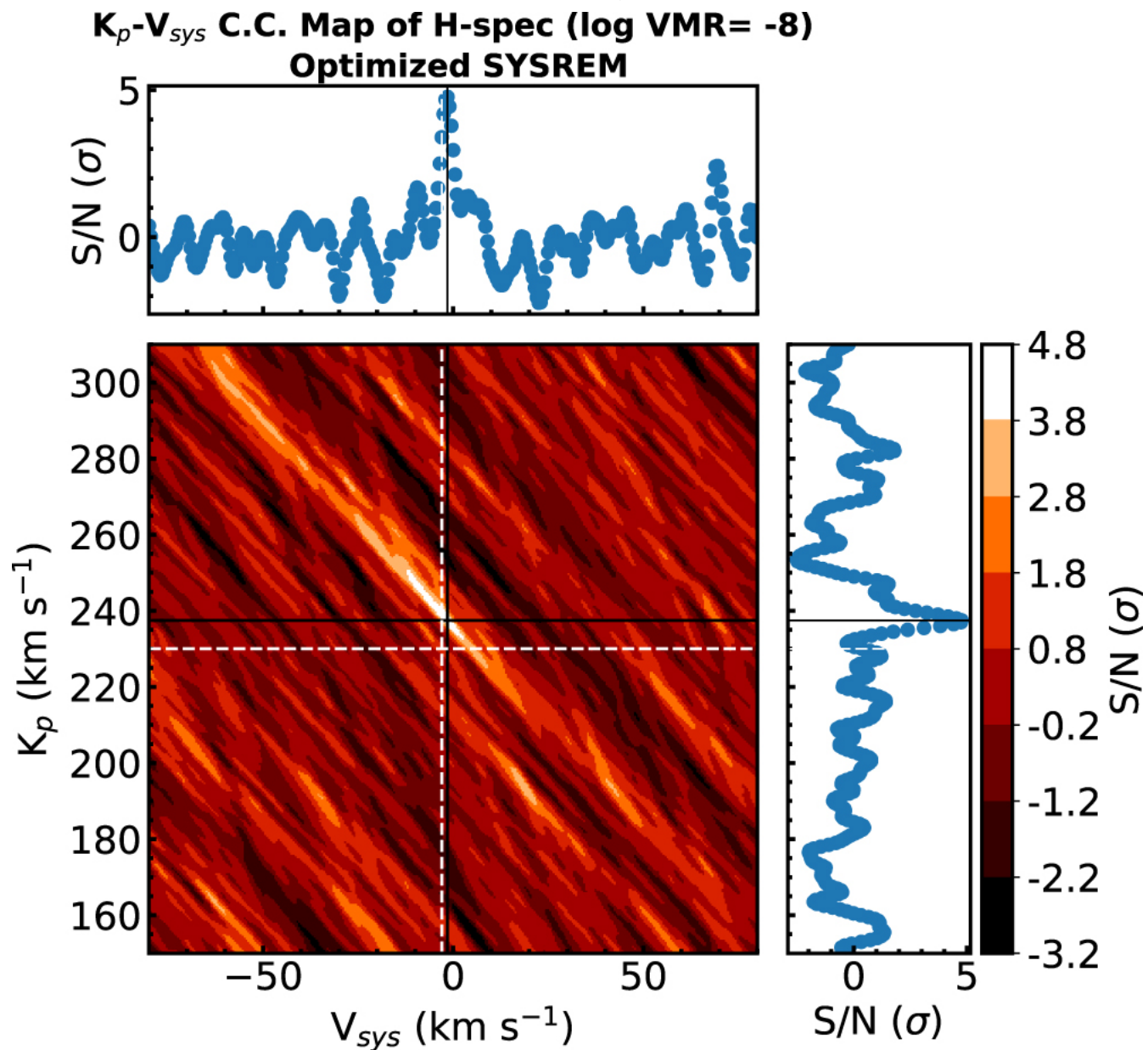
Figure 14. from High-resolution Spectroscopic Detection of TiO and a Stratosphere in the Day-side of WASP-33b null 2017 AJ 154 221 doi:10.3847/1538-3881/aa9433 https://dx.doi.org/10.3847/1538-3881/aa9433
