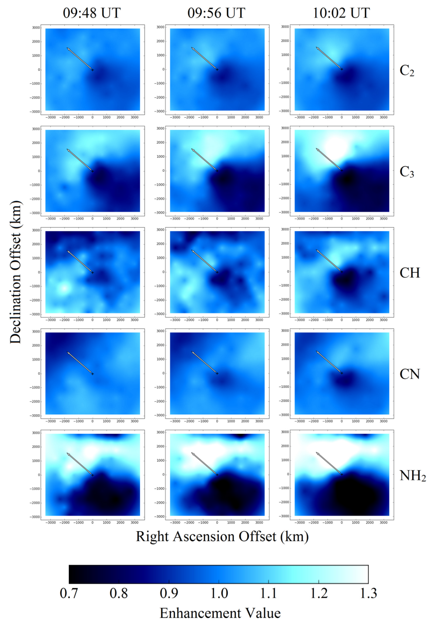
Figure 8. from Jet Morphology and Coma Analysis of Comet 103P/Hartley 2 null 2017 AJ 154 219 doi:10.3847/1538-3881/aa9382 https://dx.doi.org/10.3847/1538-3881/aa9382 © 2017. The American Astronomical Society. All rights reserved.
