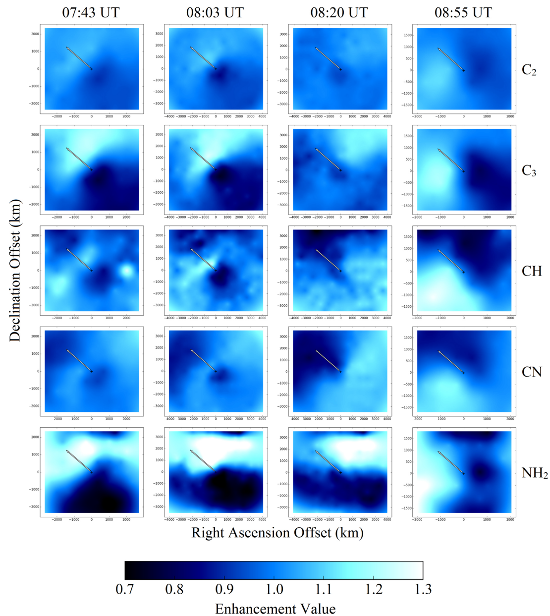
Figure 6. from Jet Morphology and Coma Analysis of Comet 103P/Hartley 2 null 2017 AJ 154 219 doi:10.3847/1538-3881/aa9382 https://dx.doi.org/10.3847/1538-3881/aa9382 © 2017. The American Astronomical Society. All rights reserved.
