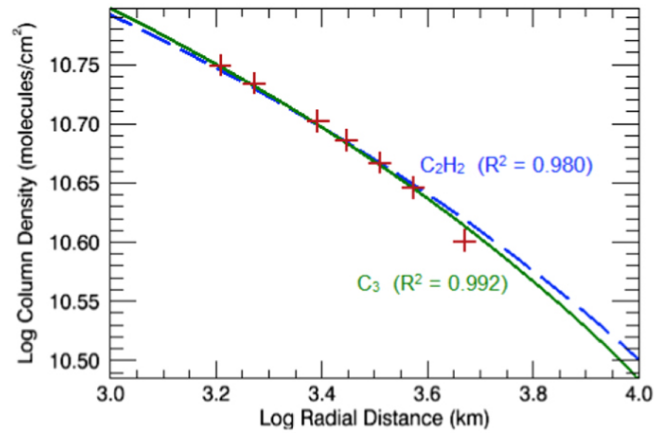
Figure 5. from Jet Morphology and Coma Analysis of Comet 103P/Hartley 2 null 2017 AJ 154 219 doi:10.3847/1538-3881/aa9382 https://dx.doi.org/10.3847/1538-3881/aa9382 © 2017. The American Astronomical Society. All rights reserved.
