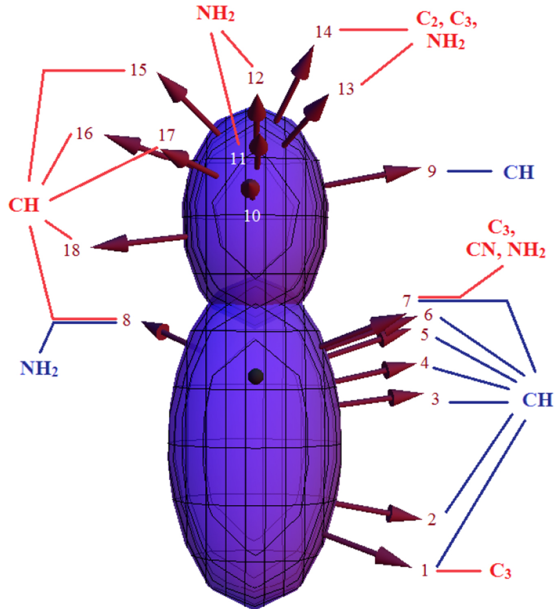
Figure 4. from Jet Morphology and Coma Analysis of Comet 103P/Hartley 2 null 2017 AJ 154 219 doi:10.3847/1538-3881/aa9382 https://dx.doi.org/10.3847/1538-3881/aa9382 © 2017. The American Astronomical Society. All rights reserved.
