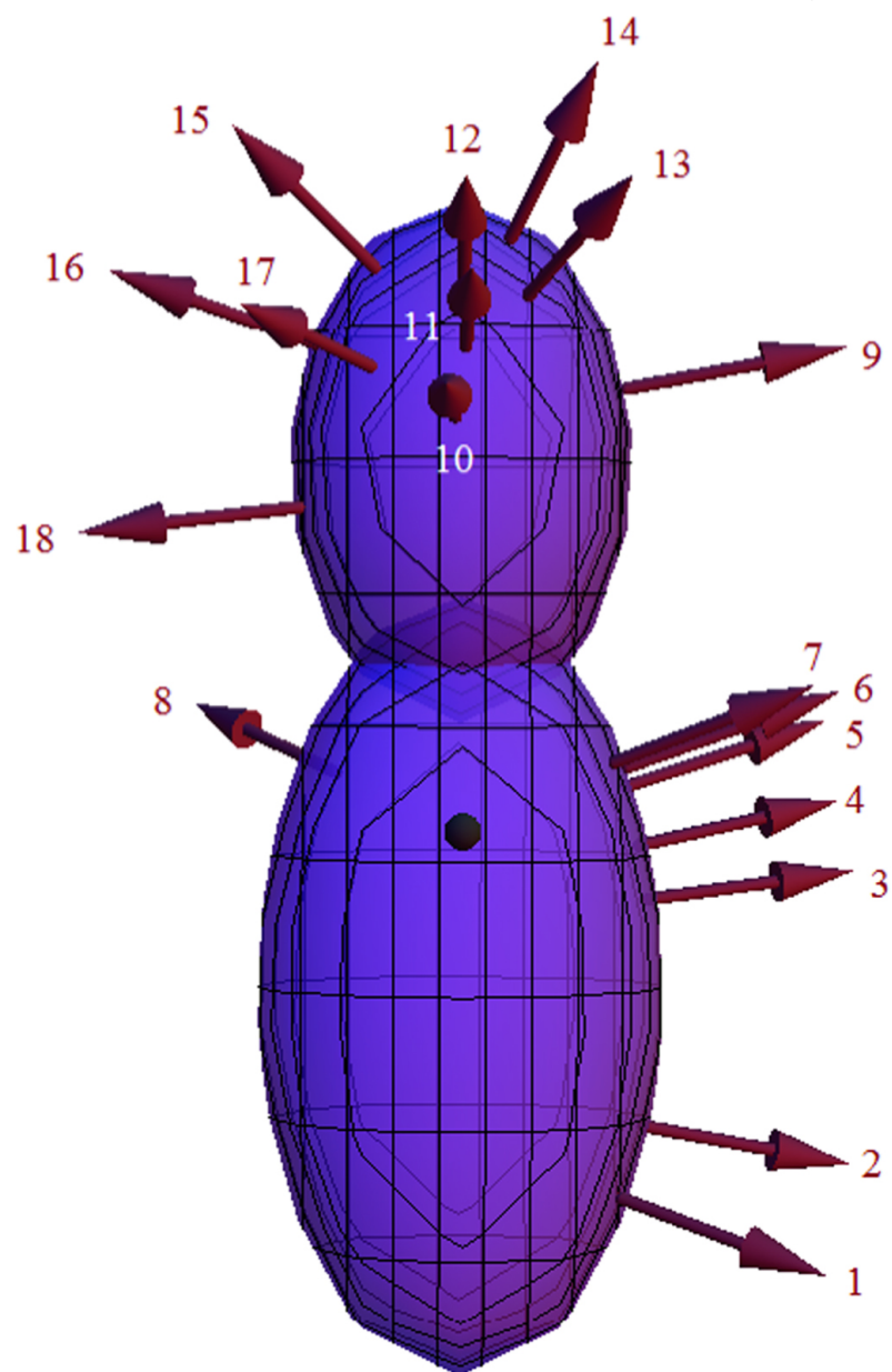
Figure 2. from Jet Morphology and Coma Analysis of Comet 103P/Hartley 2 null 2017 AJ 154 219 doi:10.3847/1538-3881/aa9382 https://dx.doi.org/10.3847/1538-3881/aa9382 © 2017. The American Astronomical Society. All rights reserved.
