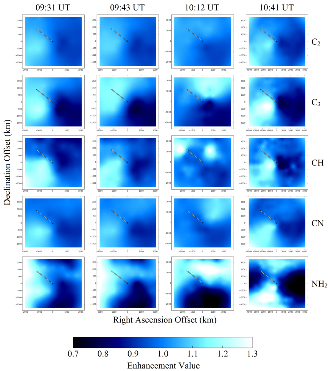
Figure 10. from Jet Morphology and Coma Analysis of Comet 103P/Hartley 2 null 2017 AJ 154 219 doi:10.3847/1538-3881/aa9382 https://dx.doi.org/10.3847/1538-3881/aa9382 © 2017. The American Astronomical Society. All rights reserved.
