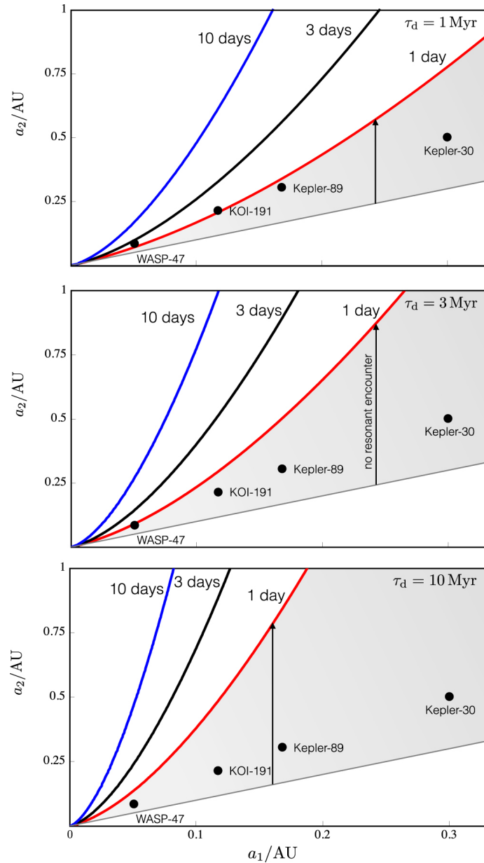
Figure 4. from A Secular Resonant Origin for the Loneliness of Hot Jupiters null 2017 AJ 154 93 doi:10.3847/1538-3881/aa8174 https://dx.doi.org/10.3847/1538-3881/aa8174 © 2017. The American Astronomical Society. All rights reserved.
