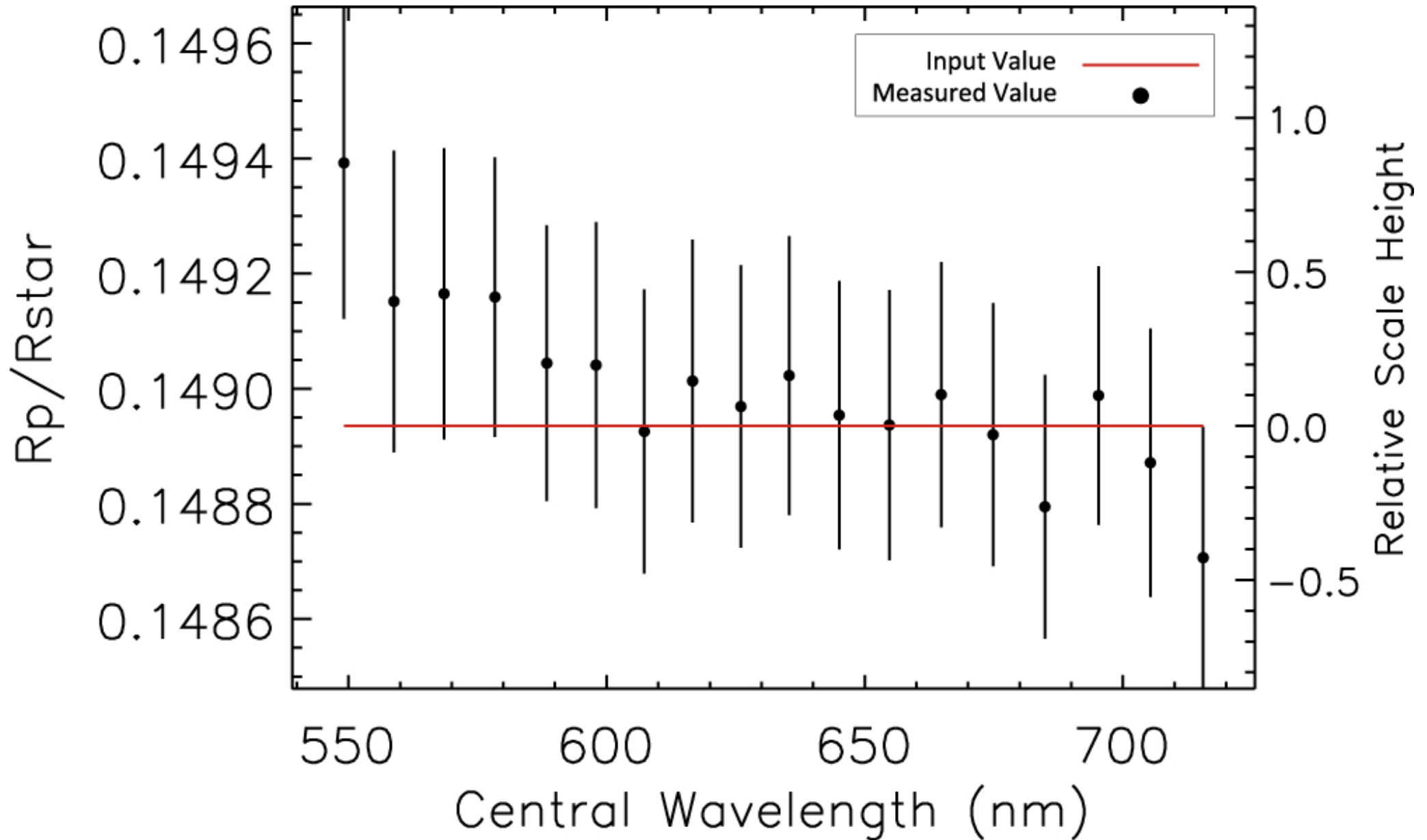
Figure 9. from Gemini/GMOS Transmission Spectral Survey: Complete Optical Transmission Spectrum of the Hot Jupiter WASP-4b null 2017 AJ 154 95 doi:10.3847/1538-3881/aa7f72 https://dx.doi.org/10.3847/1538-3881/aa7f72 © 2017. The American Astronomical Society. All rights reserved.
