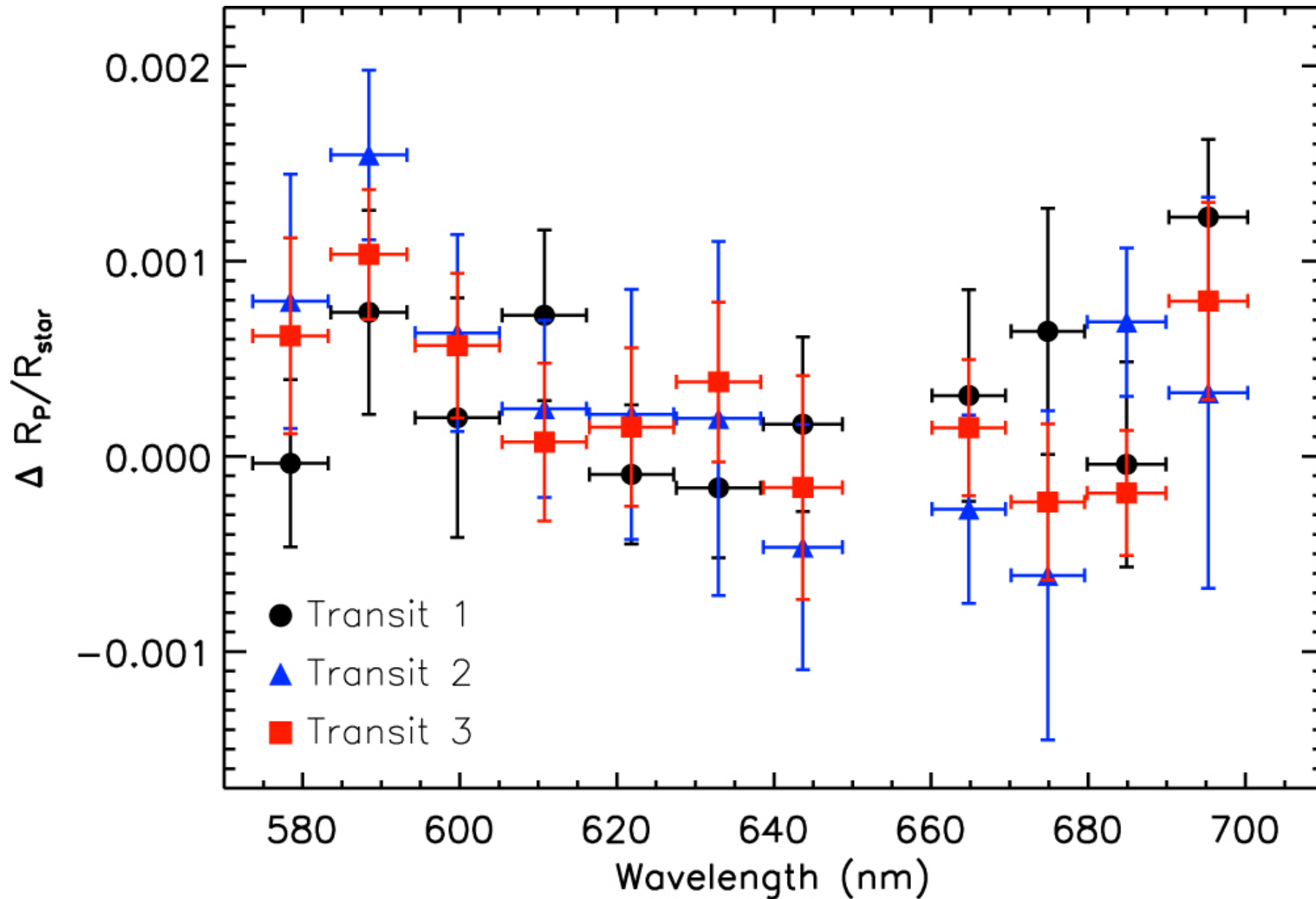
Figure 8. from Gemini/GMOS Transmission Spectral Survey: Complete Optical Transmission Spectrum of the Hot Jupiter WASP-4b null 2017 AJ 154 95 doi:10.3847/1538-3881/aa7f72 https://dx.doi.org/10.3847/1538-3881/aa7f72 © 2017. The American Astronomical Society. All rights reserved.
