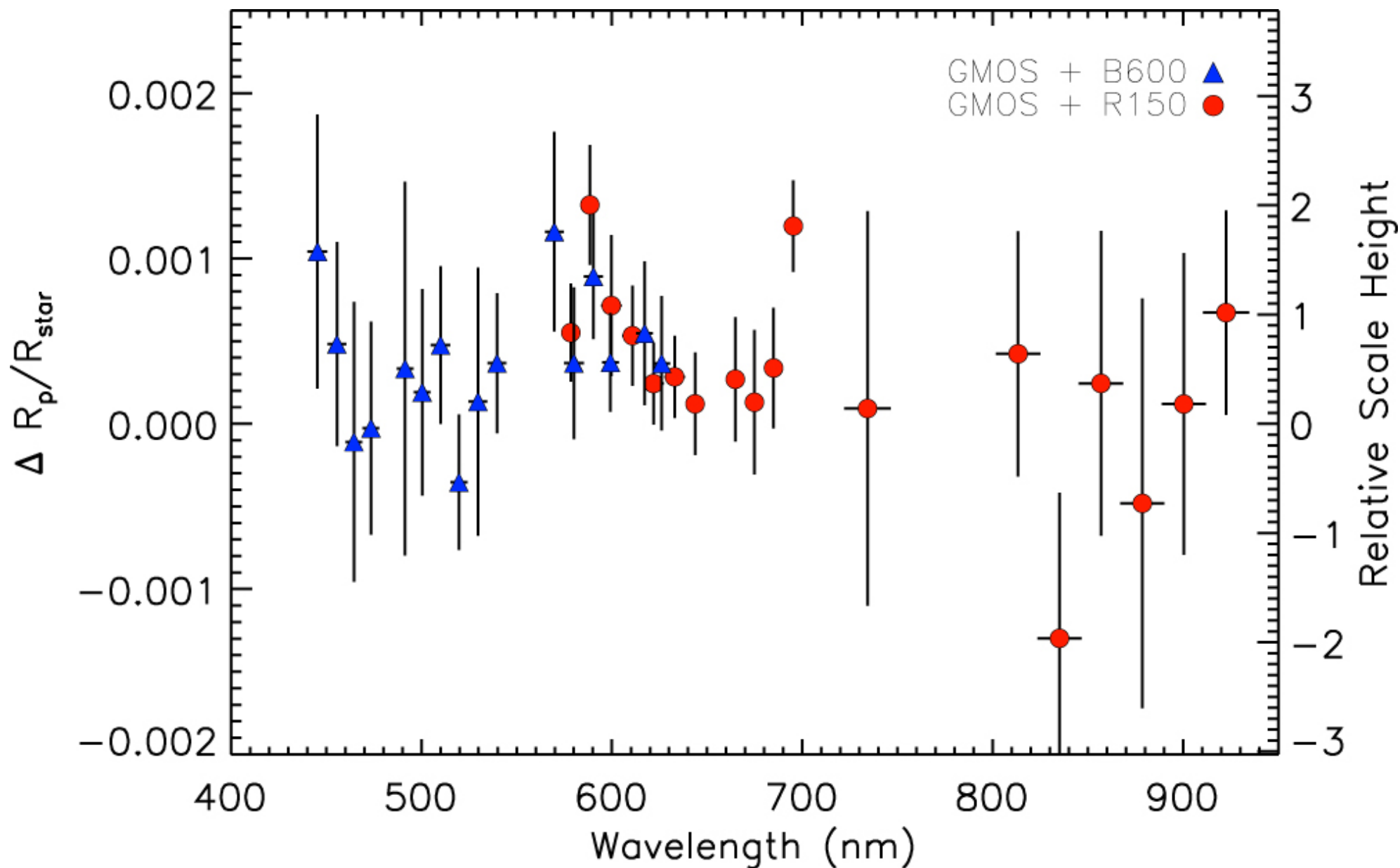
Figure 7. from Gemini/GMOS Transmission Spectral Survey: Complete Optical Transmission Spectrum of the Hot Jupiter WASP-4b null 2017 AJ 154 95 doi:10.3847/1538-3881/aa7f72 https://dx.doi.org/10.3847/1538-3881/aa7f72 © 2017. The American Astronomical Society. All rights reserved.
