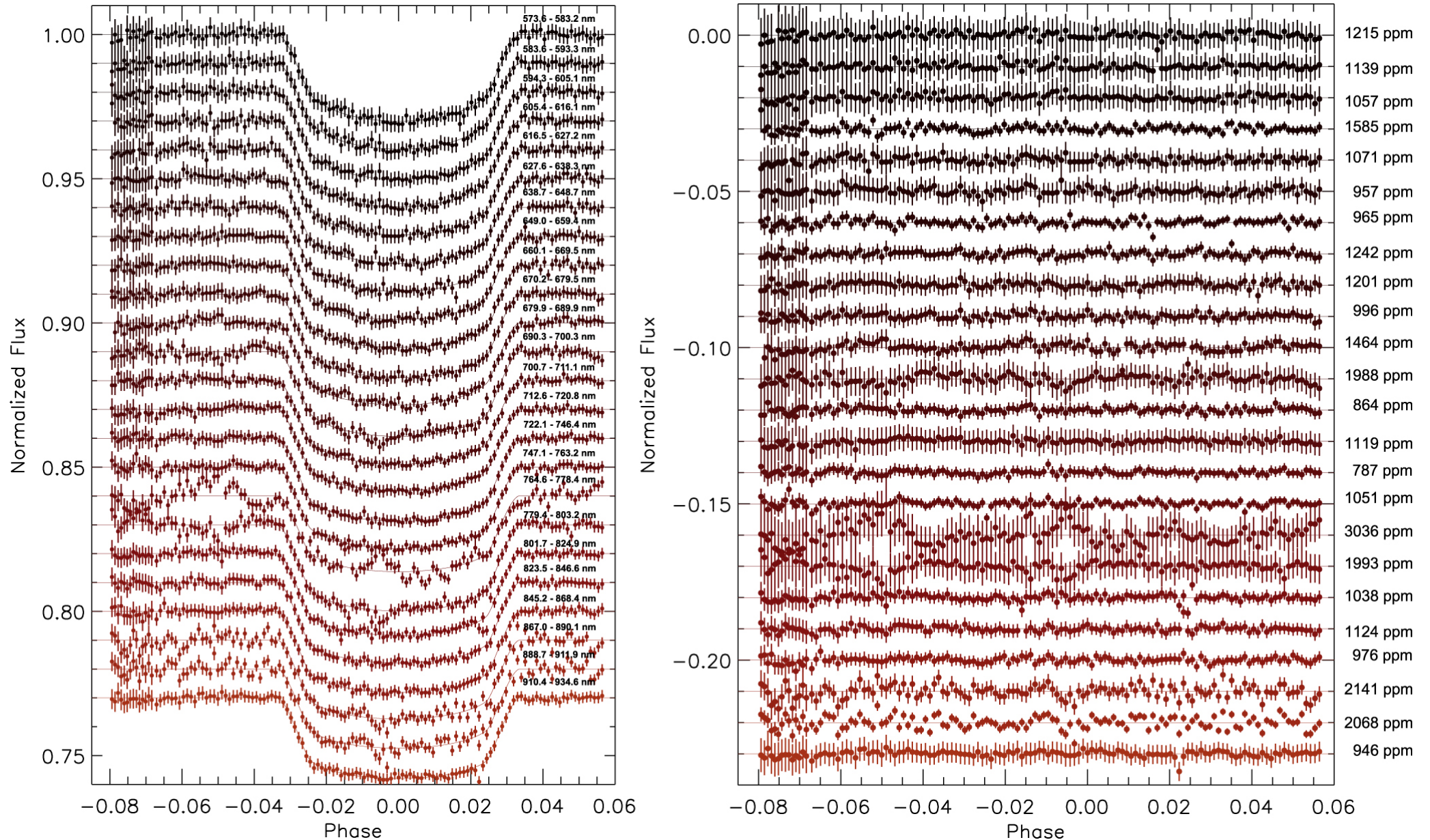
Figure 6. from Gemini/GMOS Transmission Spectral Survey: Complete Optical Transmission Spectrum of the Hot Jupiter WASP-4b null 2017 AJ 154 95 doi:10.3847/1538-3881/aa7f72 https://dx.doi.org/10.3847/1538-3881/aa7f72 © 2017. The American Astronomical Society. All rights reserved.
