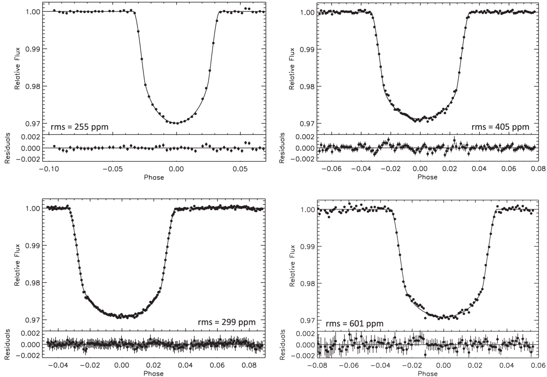
Figure 3. from Gemini/GMOS Transmission Spectral Survey: Complete Optical Transmission Spectrum of the Hot Jupiter WASP-4b null 2017 AJ 154 95 doi:10.3847/1538-3881/aa7f72 https://dx.doi.org/10.3847/1538-3881/aa7f72 © 2017. The American Astronomical Society. All rights reserved.
