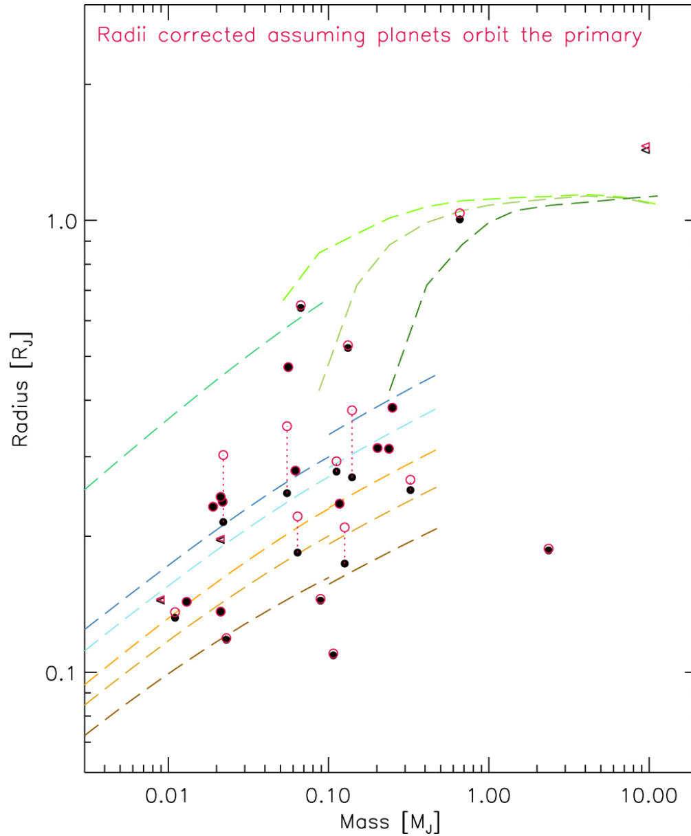
Figure 3. from The Densities of Planets in Multiple Stellar Systems null 2017 AJ 154 66 doi:10.3847/1538-3881/aa7b70 https://dx.doi.org/10.3847/1538-3881/aa7b70 © 2017. The American Astronomical Society. All rights reserved.
