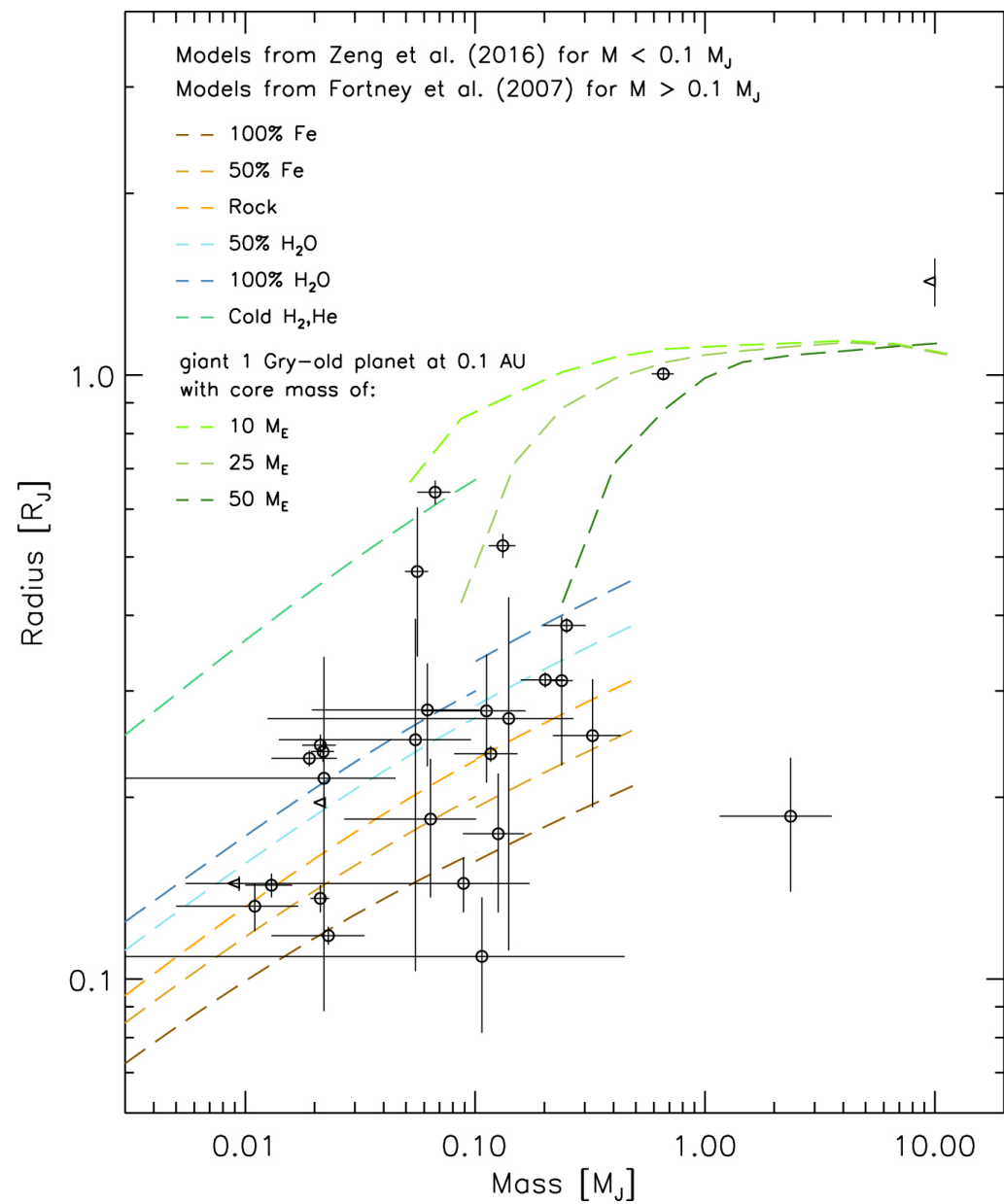
Figure 2. from The Densities of Planets in Multiple Stellar Systems null 2017 AJ 154 66 doi:10.3847/1538-3881/aa7b70 https://dx.doi.org/10.3847/1538-3881/aa7b70 © 2017. The American Astronomical Society. All rights reserved.
