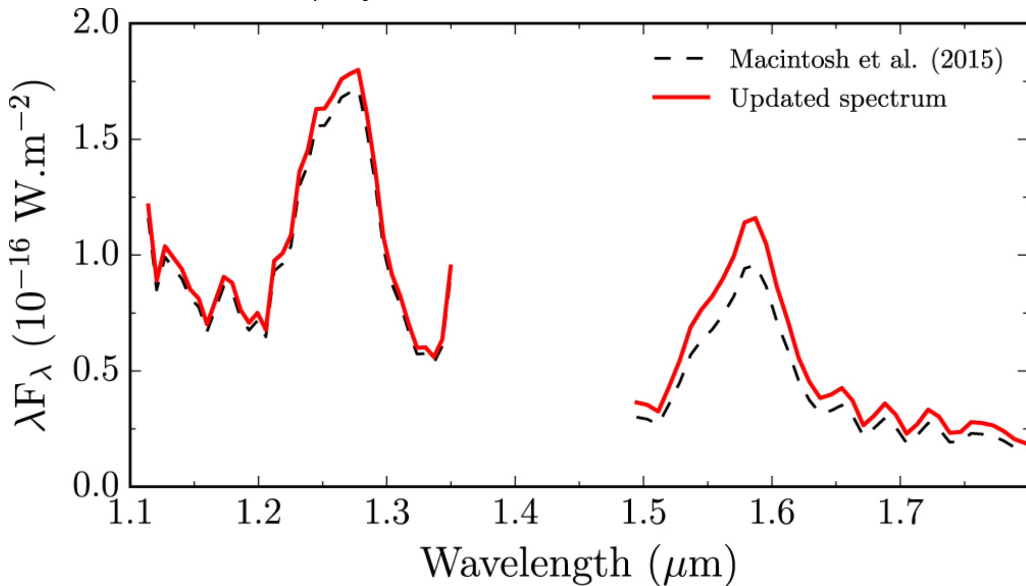
Figure 2. from Characterizing 51 Eri b from 1 to 5 m: A Partly Cloudy Exoplanet null 2017 AJ 154 10 doi:10.3847/1538-3881/aa74db https://dx.doi.org/10.3847/1538-3881/aa74db © 2017. The American Astronomical Society. All rights reserved.
