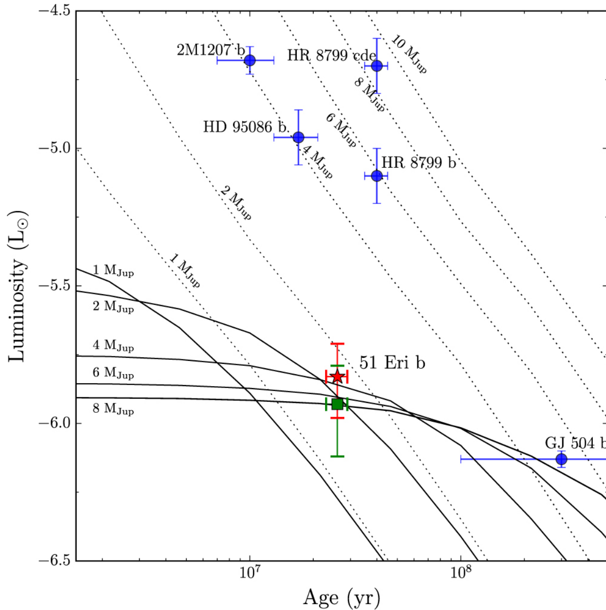
Figure 16. from Characterizing 51 Eri b from 1 to 5 m: A Partly Cloudy Exoplanet null 2017 AJ 154 10 doi:10.3847/1538-3881/aa74db https://dx.doi.org/10.3847/1538-3881/aa74db © 2017. The American Astronomical Society. All rights reserved.
